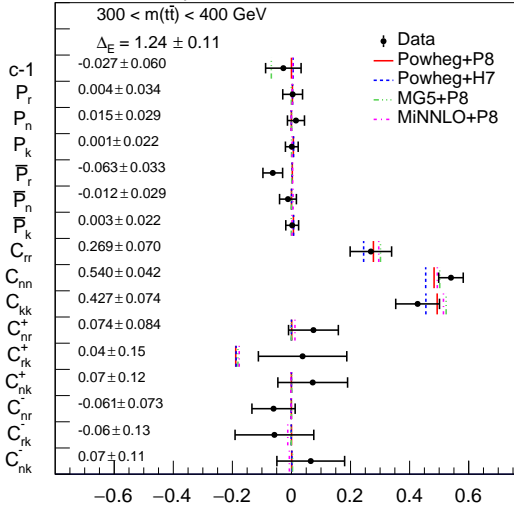
CMS Preliminary 138 fb -1 (13 TeV)
