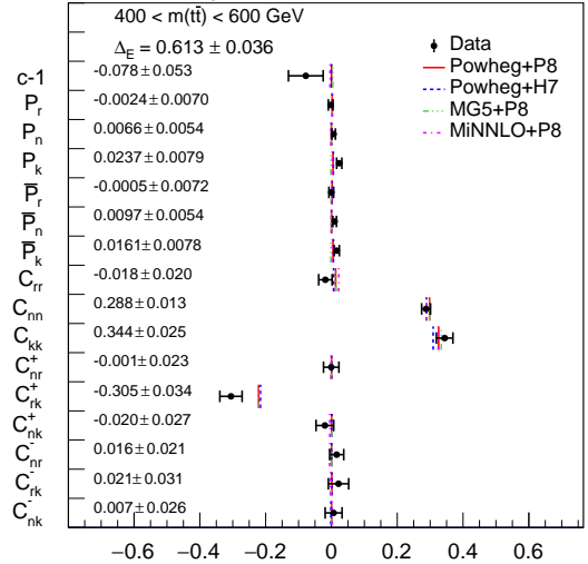
CMS Preliminary 138 fb -1 (13 TeV)
