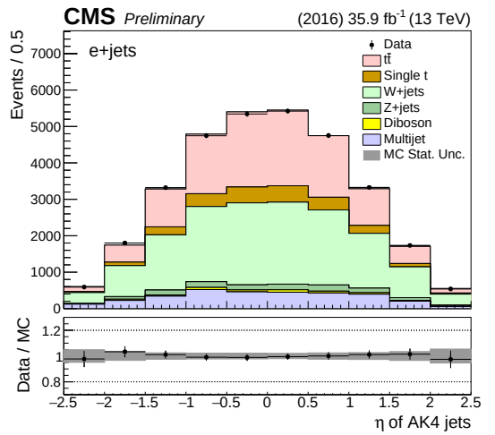
(b) 0t, e+jets
