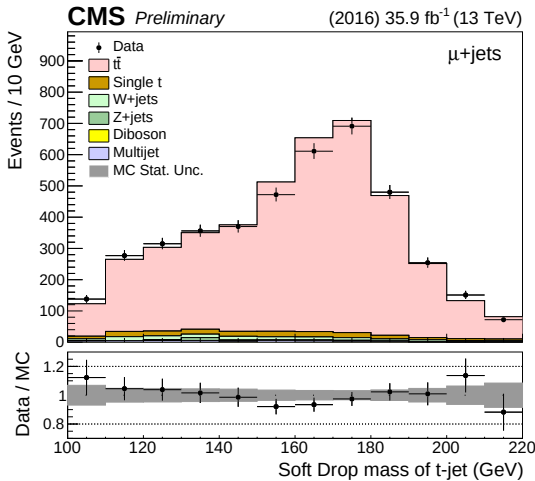
(e) 1t1b, \mu +jets
