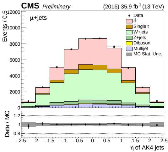
(a) 0t, \mu +jets
