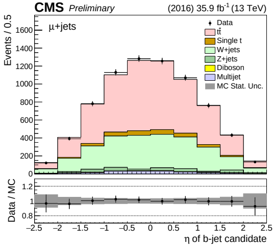
(c) 1t0b, \mu +jets
