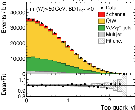
CMS Preliminary (e, \mu )+2j1b, 36fb -1 (13TeV)
