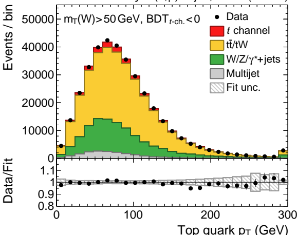
CMS Preliminary (e, \mu )+2j1b, 36fb -1 (13TeV)
