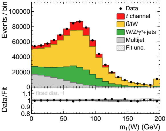
CMS Preliminary (e, \mu )+2j1b, 36fb -1 (13TeV)
