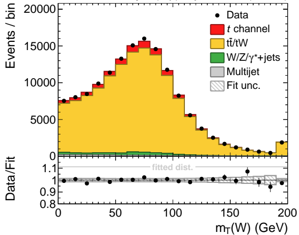
CMS Preliminary (e, \mu )+3j2b, 36fb -1 (13TeV)
