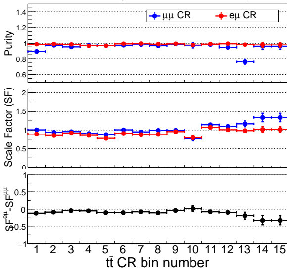
CMS Preliminary
