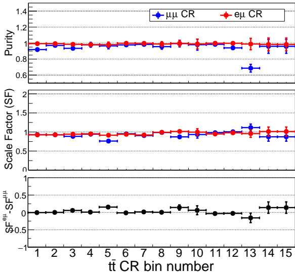
CMS Preliminary
