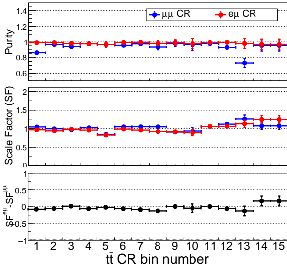
59.7 fb -1 (13 TeV)
