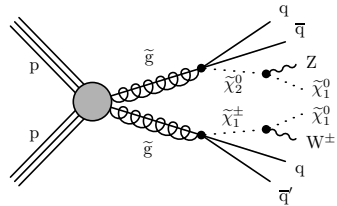
(c) T5qqqqWZ
