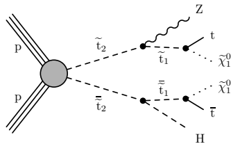
(e) T6ttHZ
