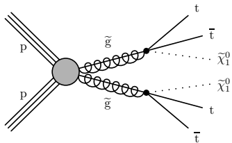
(a) T1tttt
