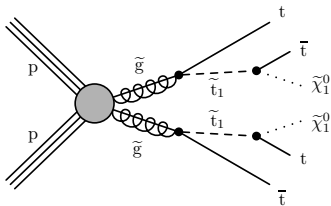
(b) T5tttt
