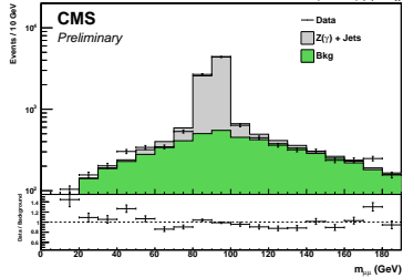
19.7 fb -1 (8 TeV) \mu\mu +bjj
