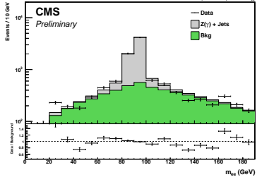
19.7 fb -1 (8 TeV) ee+bjj
