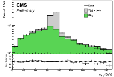
19.7 fb -1 (8 TeV) e \gamma +jjj
