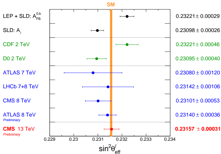
Figure 1: Comparison of the \sin^2 \theta_{\text{eff}}^l values measured in this analysis with previous measurements and the SM prediction.
