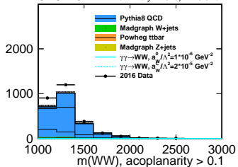
CMS+TOTEM Preliminary 2016, L = 9.9 fb -1
