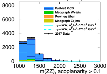
CMS+TOTEM Preliminary 2017, L = 37.2 fb -1
