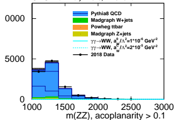
CMS Preliminary 2018, L = 52.9 fb -1
