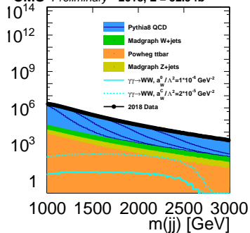
CMS Preliminary 2018, L = 52.9 fb -1
