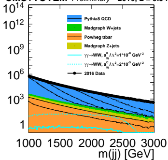
CMS+TOTEM Preliminary 2016, L = 9.9 fb -1
