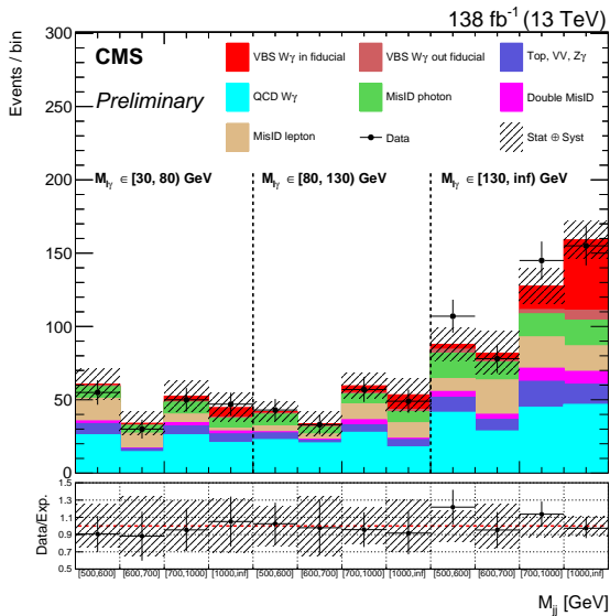
(b) Endcap
