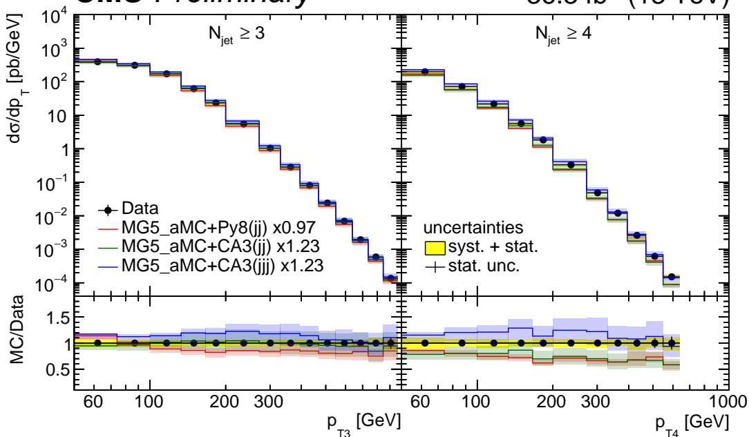
(b) Third and fourth leading jet p_T distributions.
