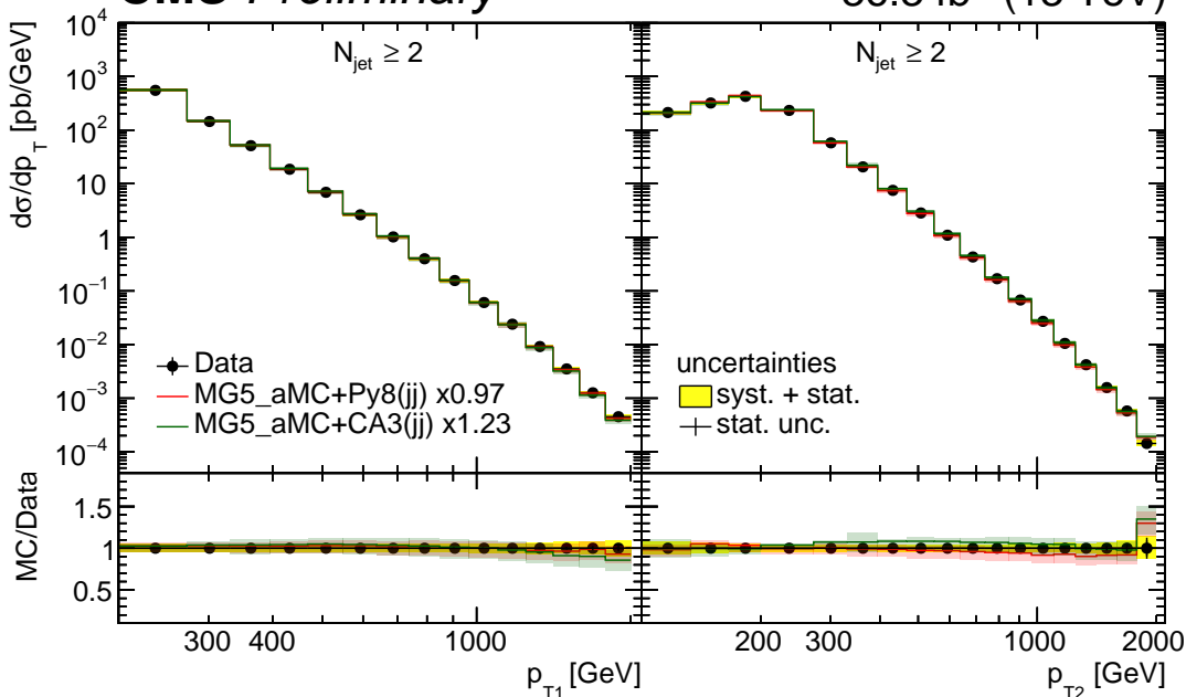
(a) Leading and second leading jet p_T distributions.
