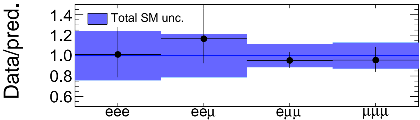
Lepton flavour composition
