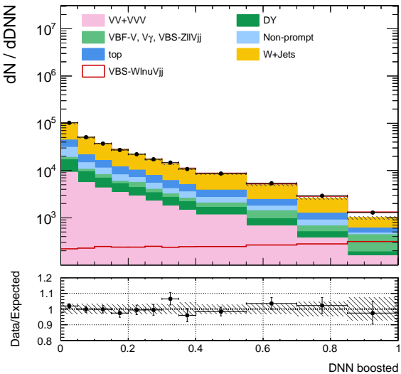
CMS Preliminary L = 137/fb (13 TeV)
