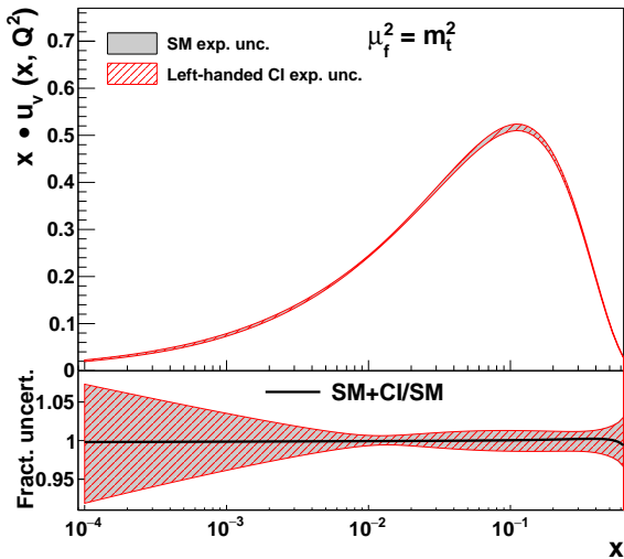
CMS Preliminary HERA+CMS 13 TeV, Hessian unc.
