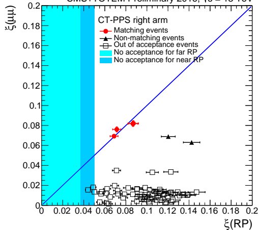
CMS+TOTEM Preliminary 2016, \sqrt{s} = 13 TeV
