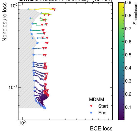
CMS Simulation Preliminary (13 TeV)
