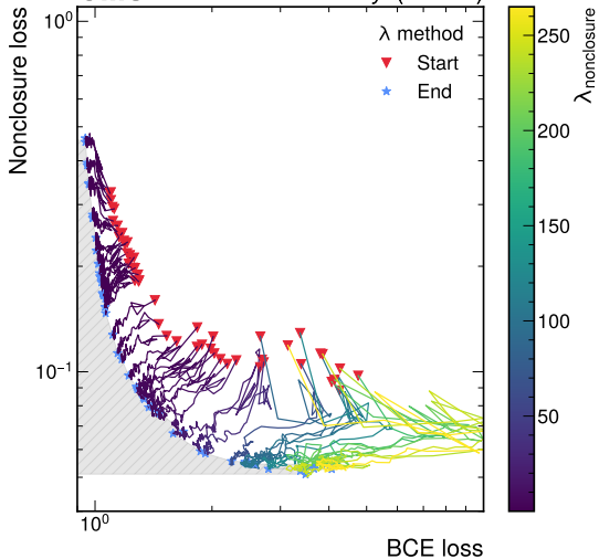
CMS Simulation Preliminary (13 TeV)
