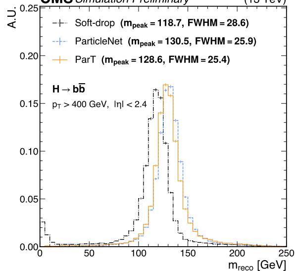
CMS Simulation Preliminary (13 TeV)
