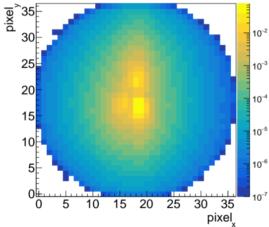
CMS Simulation Preliminary
