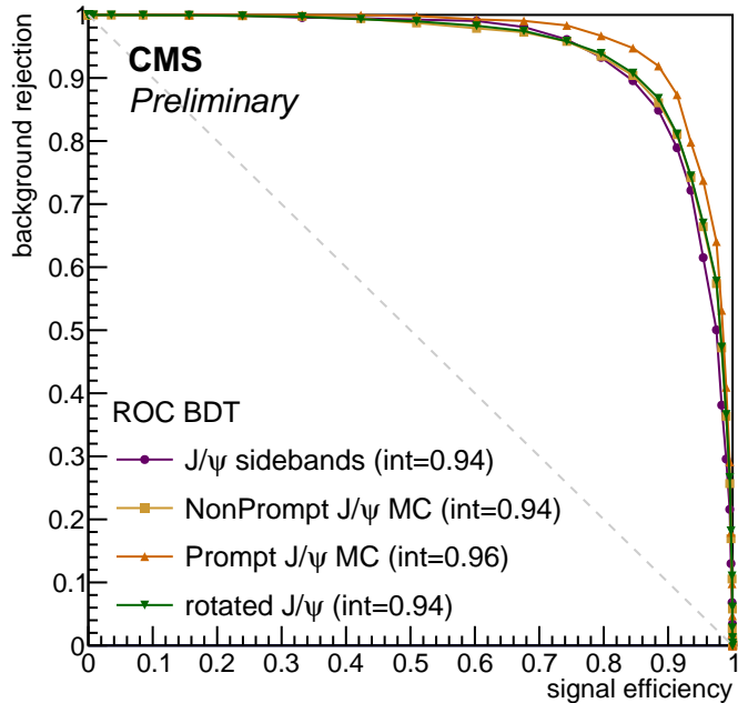
ROC curve (lower cut)
