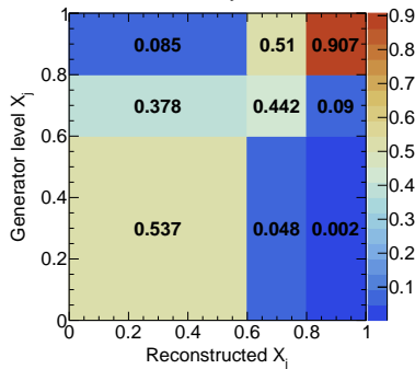
CMS Simulation Preliminary
