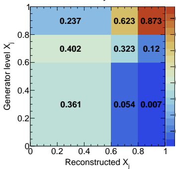
CMS Simulation Preliminary
