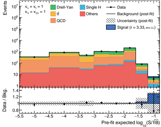
CMS Preliminary bb \tau\tau ( \tau\tau channel), 138 fb ^{-1} (13 TeV)
