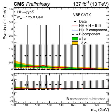
(b) VBF CAT 0
