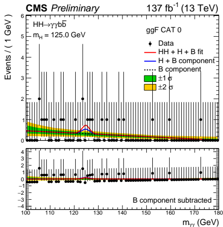
(a) ggF CAT 0
