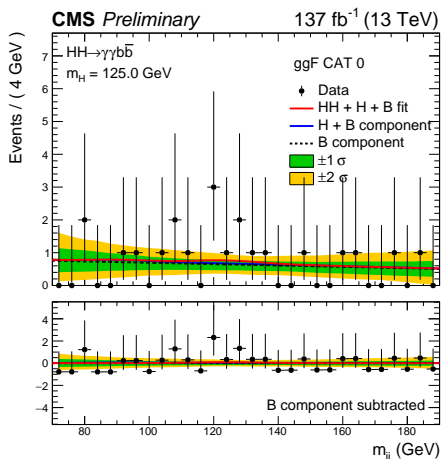
(c) ggF CAT 0
