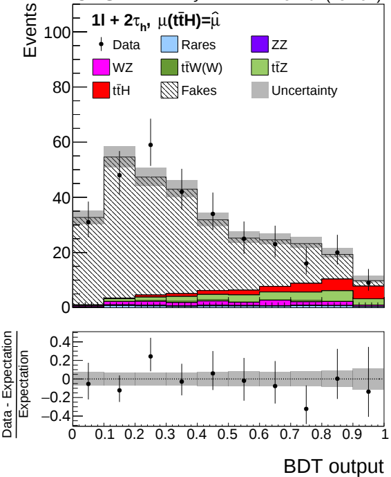
CMS Preliminary 137 fb -1 (13 TeV)
