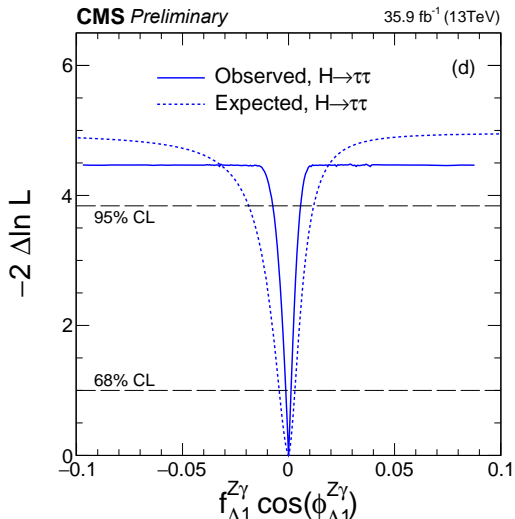
Observed (solid) and expected (dashed) likelihood scans of f_{a3} \cos(\phi_{a3}) (a), f_{a2} \cos(\phi_{a2}) (b), f_{\Lambda 1} \cos(\phi_{\Lambda 1}) (c), and f_{\Lambda 1}^{Z\gamma} \cos(\phi_{\Lambda 1}^{Z\gamma}) (d).
