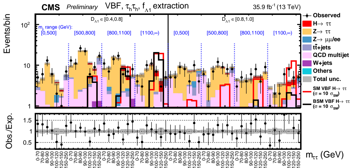
Observed and expected distributions in the VBF category in bins of m_{\tau\tau} , m_{ij} and D_{\Delta 1} for the \mu\tau_h + e\tau_h + e\mu (top) and \tau_h\tau_h (middle and bottom) decay channels.
