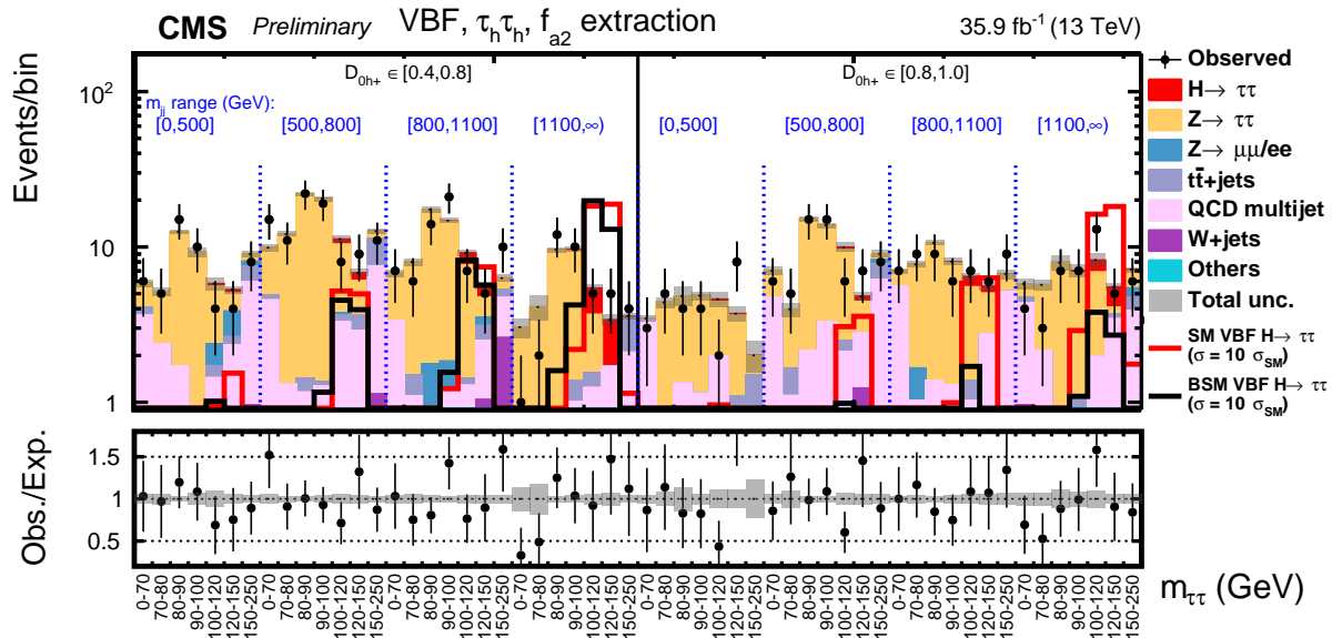
Observed and expected distributions in the VBF category in bins of m_{\tau\tau} , m_{jj} and D_{0h^+} for the \mu\tau_h + e\tau_h + e\mu (top) and \tau_h\tau_h (middle and bottom) decay channels.
