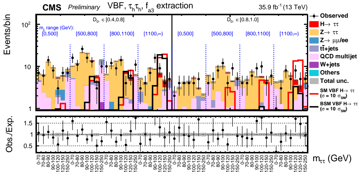
Observed and expected distributions in the VBF category in bins of m_{\tau\tau} , m_{ij} and D_{0^-} for the \mu\tau_h + e\tau_h + e\mu (top) and \tau_h\tau_h (middle and bottom) decay channels.
