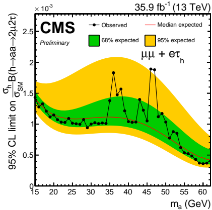
(b) \mu\mu e\tau_h
