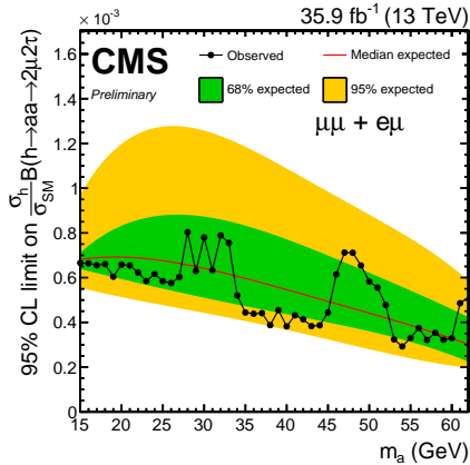
(a) \mu\mu e\mu
