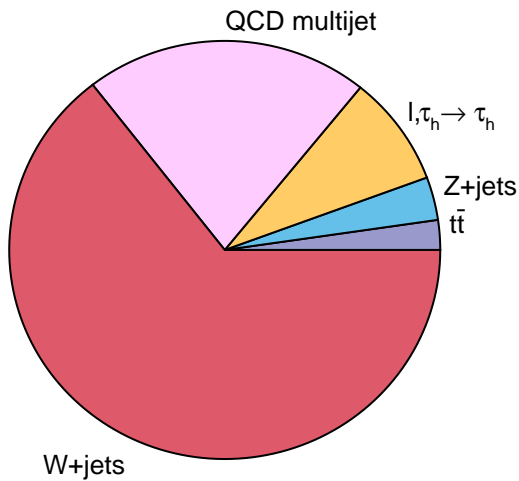
e \tau_h No B-tag Loose-m \tau
