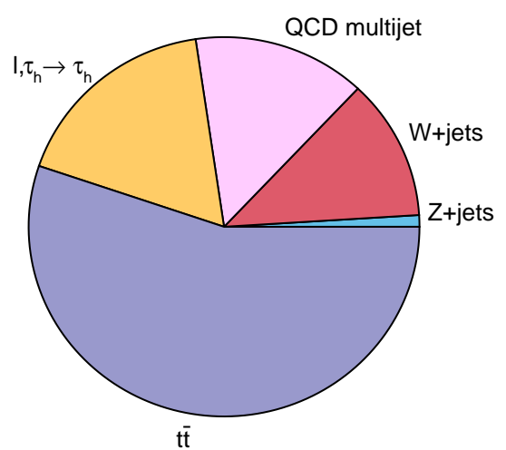
e \tau_h B-tag Loose-m \tau
