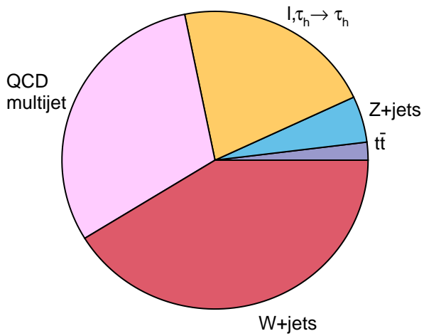
e \tau_h No B-tag Tight-m \tau
