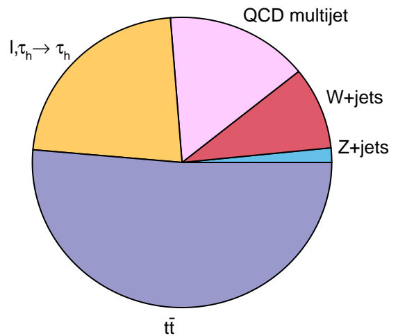
e \tau_h B-tag Tight-m \tau
