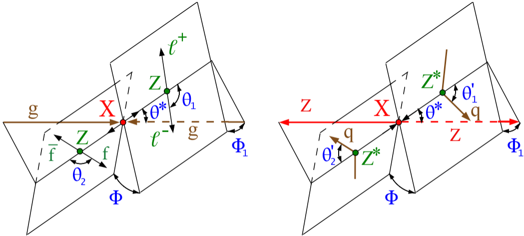
Illustration of an X boson production from ggH, gg \rightarrow X \rightarrow ZZ \rightarrow (l^+ l^-)(f \bar{f}) (left) and VBF qq' \rightarrow qq'X \rightarrow qq'ZZ (right).
