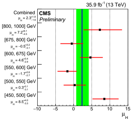
(a) \mu_H , with \mu_Z profiled
