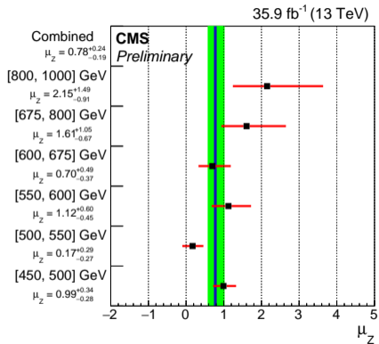
(b) \mu_Z , with \mu_H profiled
