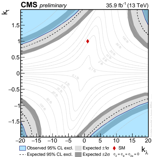
(b) Exclusion in (k_\lambda, k_t) plane
