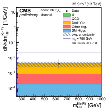
(e) boosted - resonant
