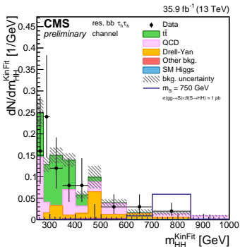
(c) resolved 2b0j - resonant
