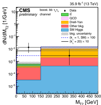
(f) boosted - non-resonant
