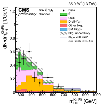
(a) resolved 1b1j - resonant
