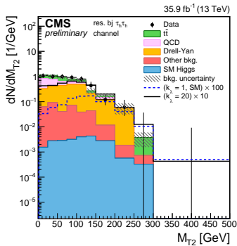
(b) resolved 1b1j - non-resonant
