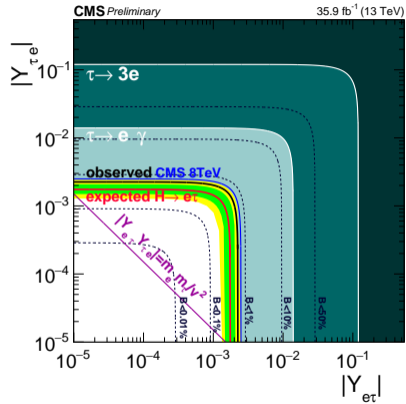
(b) Constraints on |Y_{e\tau}|, |Y_{\tau e}|
