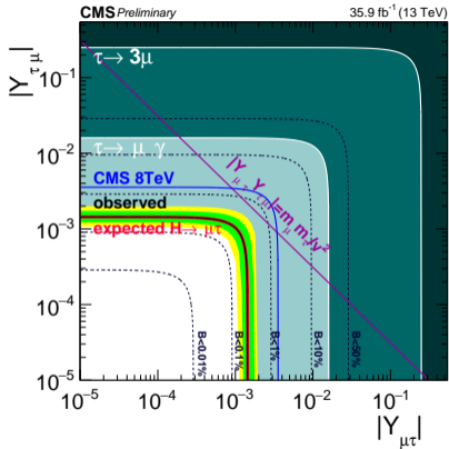
(a) Constraints on |Y_{\mu\tau}|, |Y_{\tau\mu}|
