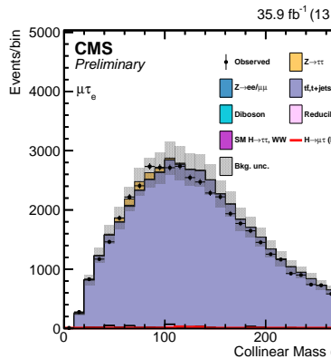
(c) t\bar{t} enriched region
