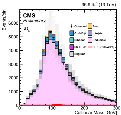
(a) Like-sign lepton region
