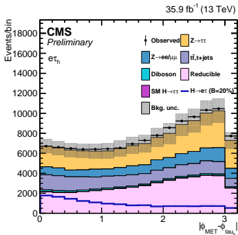
(b) \Delta\phi(\tau, E_T^{\text{miss}})
