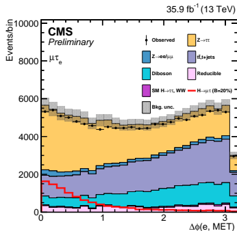
(a) \Delta\phi(e, E_T^{\text{miss}})
