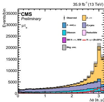
(c) \Delta\phi(e, \mu)
