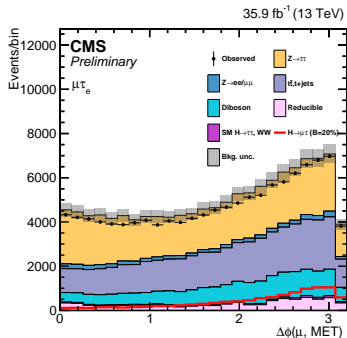
(b) \Delta\phi(\mu, E_T^{\text{miss}})
