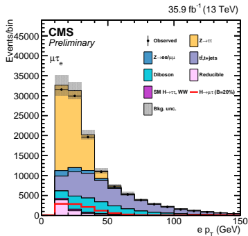
(b) e p_T
