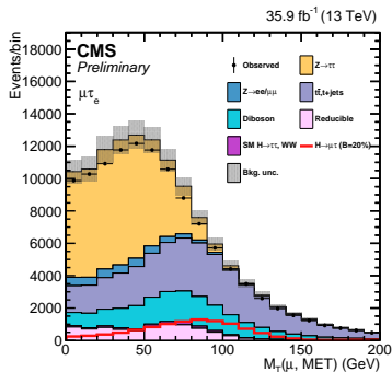
(c) M_T(\mu, E_T^{\text{miss}})
