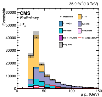
(a) \mu p_T
