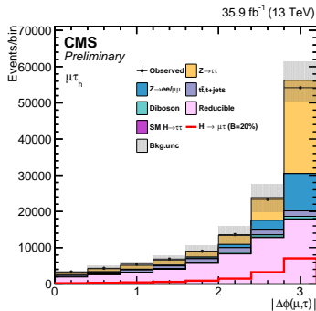
(a) \Delta\phi(\mu, \tau)
