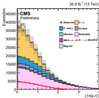
(c) \Delta\eta(\mu, \tau)
