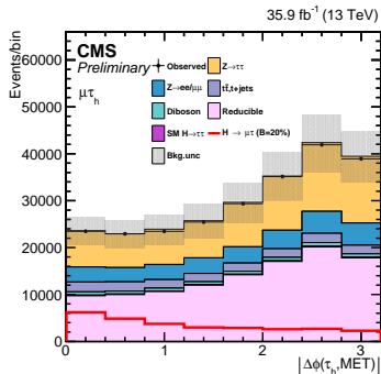
(b) \Delta\phi(\tau, E_T^{\text{miss}})
