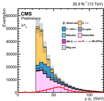
(a) \mu p_T
