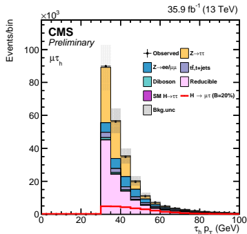
(b) \tau p_T
