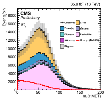
(c) M_T(\tau, E_T^{\text{miss}})
