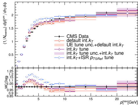
TransMAX charged-particle density, \sqrt{s} = 13 TeV
