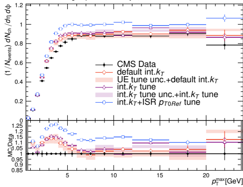
TransMIN charged-particle density, \sqrt{s} = 13 TeV
