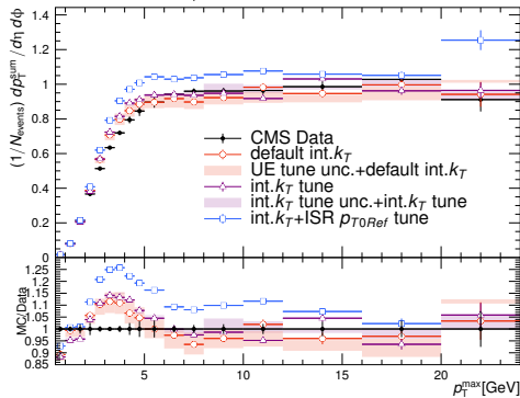
TransMIN charged-particle density, \sqrt{s} = 13 TeV
