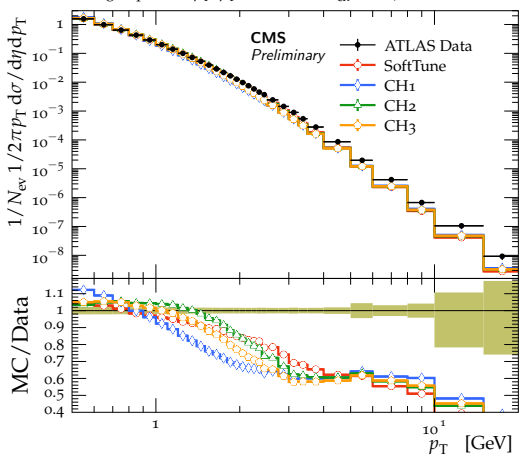
Charged particle p_T , p_T > 500 MeV, N_{ch} \geq 6 , \sqrt{s} = 900 GeV
