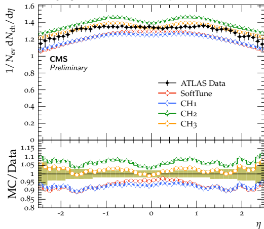
Charged particle \eta , p_T > 500 MeV, N_{ch} \geq 6 , \sqrt{s} = 900 GeV
