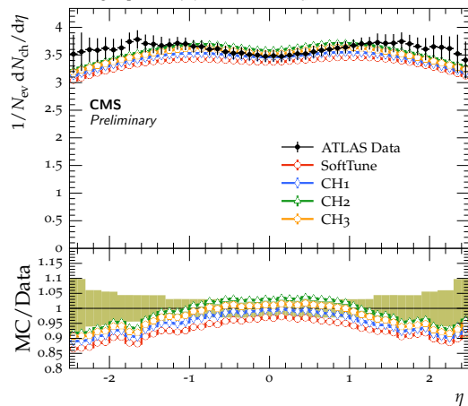
Charged particle \eta , p_T > 100 MeV, N_{ch} \geq 20 , \sqrt{s} = 900 GeV
