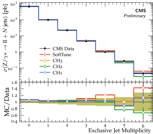
Z+jets, exclusive jet multiplicity, \sqrt{s} = 13 TeV
