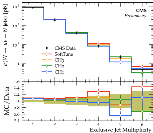
W+jets, exclusive jet multiplicity, \sqrt{s} = 13 TeV
