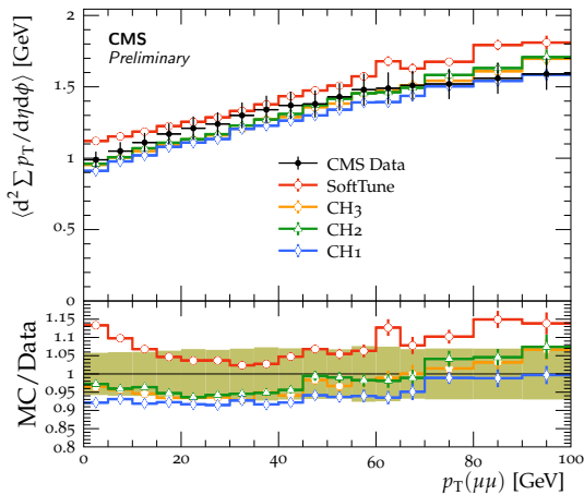
Away charged p_T^{\text{sum}} density \sqrt{s} = 13 TeV
