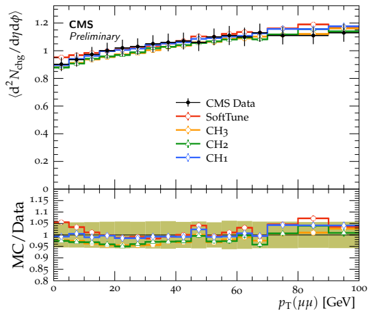
Away charged-particle density \sqrt{s} = 13 TeV
