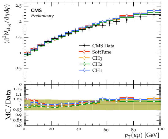
Transverse charged-particle density \sqrt{s} = 13 TeV
