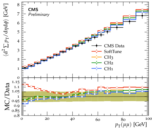
Transverse charged p_T^{\text{sum}} density \sqrt{s} = 13 TeV
