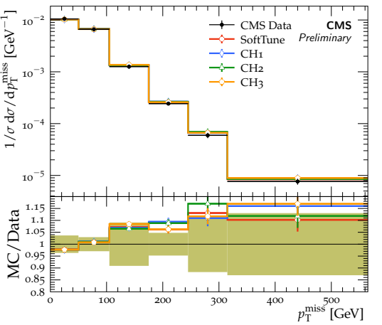
p_T^{\text{miss}} in lepton+jets t\bar{t} events, \sqrt{s} = 13 TeV
