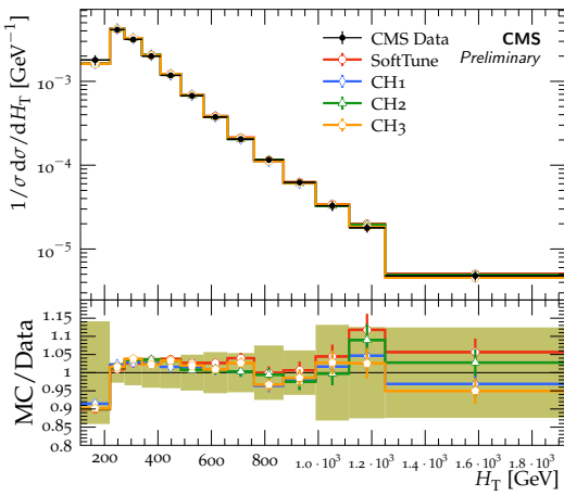
H_T in lepton+jets t\bar{t} events, \sqrt{s} = 13 TeV
