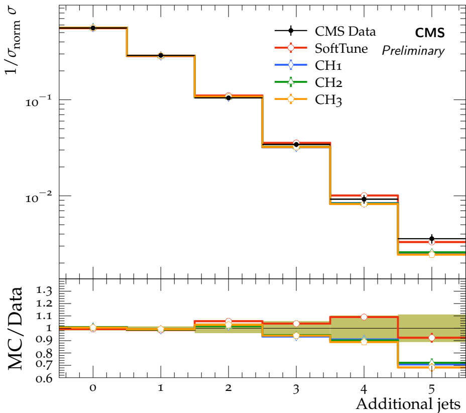
Jet multiplicity in lepton+jets t\bar{t} events, \sqrt{s} = 13 TeV
