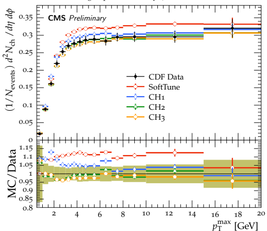
TransMin charged-particle density \sqrt{s} = 1.96 TeV
