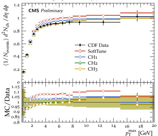
TransMax charged-particle density \sqrt{s} = 1.96 TeV
